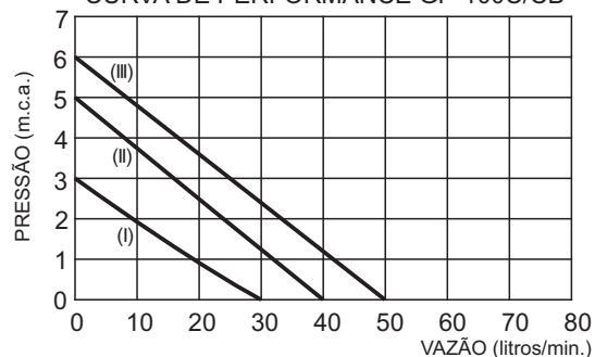
CURVA DE PERFORMANCE GP-100C/CB
