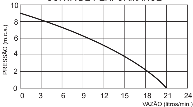
CURVA DE PERFORMANCE
