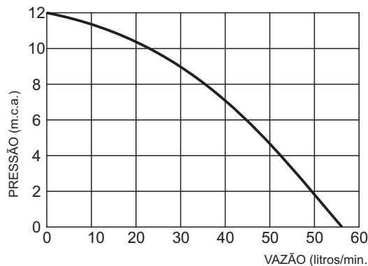
CURVA DE PERFORMANCE GP-270P
